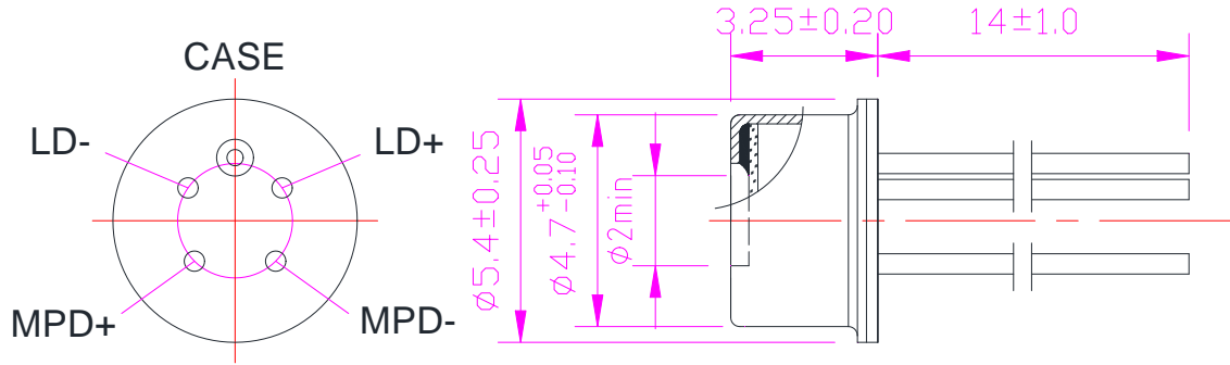
BOTTOM VIEW
